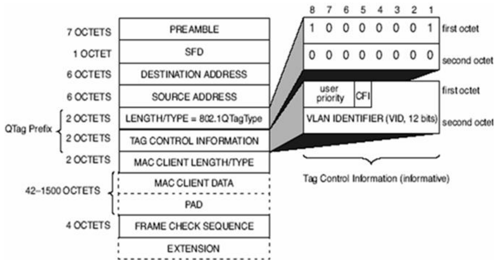
Figure 5-4 Tagged Frame
